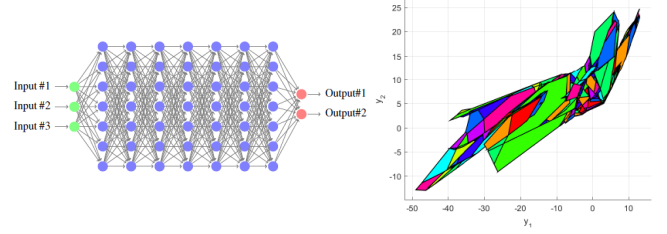
Fig. 2. Example output reachable set computation for a neural network with 3 inputs, 2 outputs, and 7 hidden layers with 7 neurons each, where all activation functions are ReLUs and all parameters of the network (weights, biases) are chosen randomly. The input set I = \{x \mid \|x\|_\infty \leq 1, x \in \mathbb{R}^3\} is a cube and convex, while the output set shown is non-convex, represented as the union of the different colored polyhedra.
