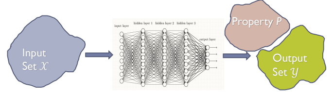
Fig. 1. Illustration of neural network reachability, where the output reachable set of a mathematical function F : \mathbb{R}^n \mapsto \mathbb{R}^m representing the neural network's behavior under a set of inputs \mathcal{X} is defined and computed in an exact or overapproximative manner. If F(\mathcal{X}) = \mathcal{Y} \subseteq \neg\mathcal{P} , then safety property \neg\mathcal{P} holds, while if \mathcal{P} \cap \mathcal{Y} \neq \emptyset , then unsafe states may be reached.
