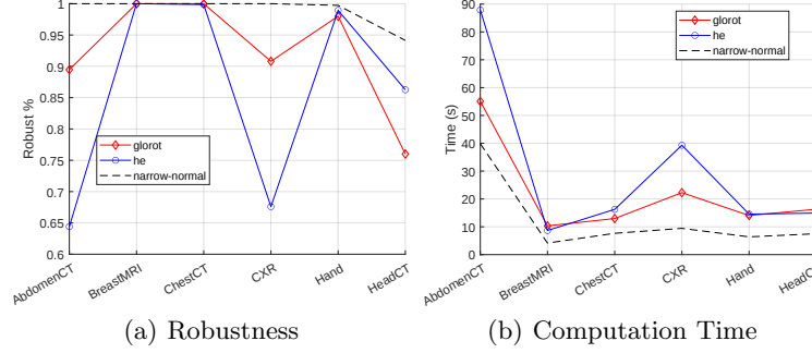
Fig. 2. MedNIST Results. Comparison across initialization schemes with respect to each image class.
